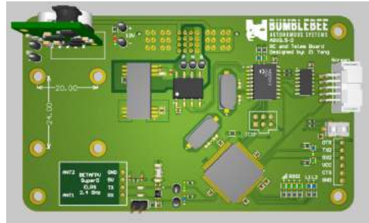
Fig. 31: 3D model of RC and Telemetry Daughter Board.
