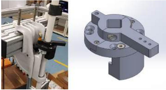
Fig. 16: Thruster setup (left) and render of mounting mechanism (right).
