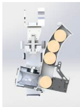
Fig. 7: Piston & Cam Mechanism.
