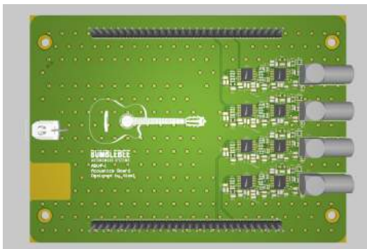
Fig. 35: 3D model of Acoustics Amplifier and Filter Board.
