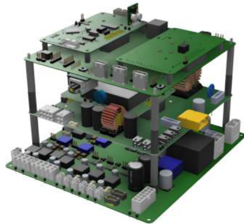
Fig. 32: 3D model of the entire Main Hull Electrical Stack.
