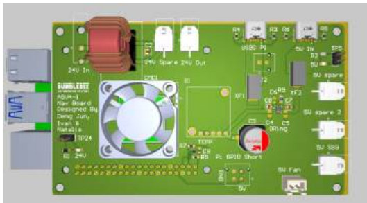
Fig. 34: 3D model of Navigation Power Board.
