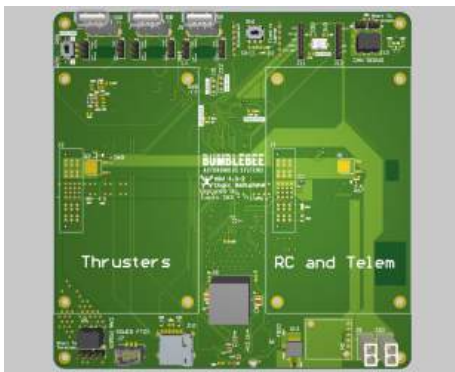
Fig. 29: 3D model of Logic Backplane.
