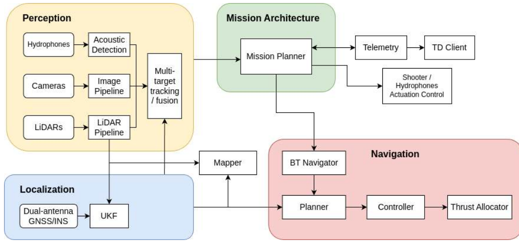
Fig. 23: High-level overview of BBASV 4.0's software architecture.
