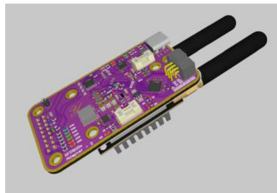
Fig. 38: 3D model of Adaptor Board for Radio Modem.
