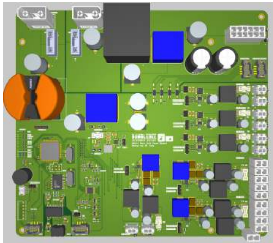
Fig. 27: 3D model of Main Hull Power Board.
