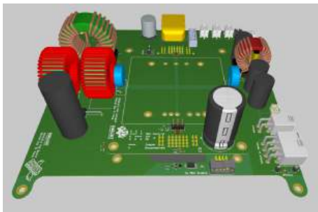
Fig. 28: 3D model of PoE 54V Stack.
