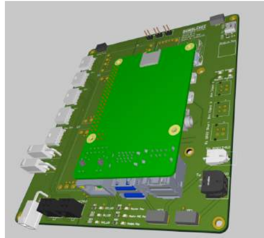
Fig. 37: 3D model of Operator Control Station 3 Board.
