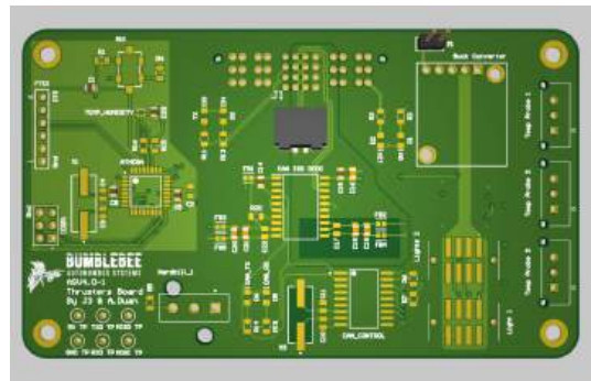
Fig. 30: 3D model of Thrusters Daughter Board.
