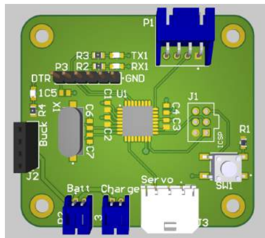
Fig. 39: 3D model of Jellyfish Floatation board.
