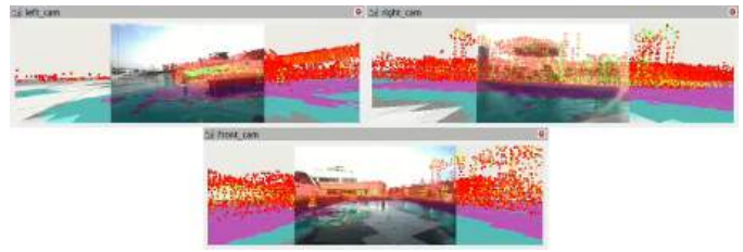
Fig. 8: Camera views (clockwise from top left: left, right, front). Coloured points overlaid on images represent fused LiDAR data.
