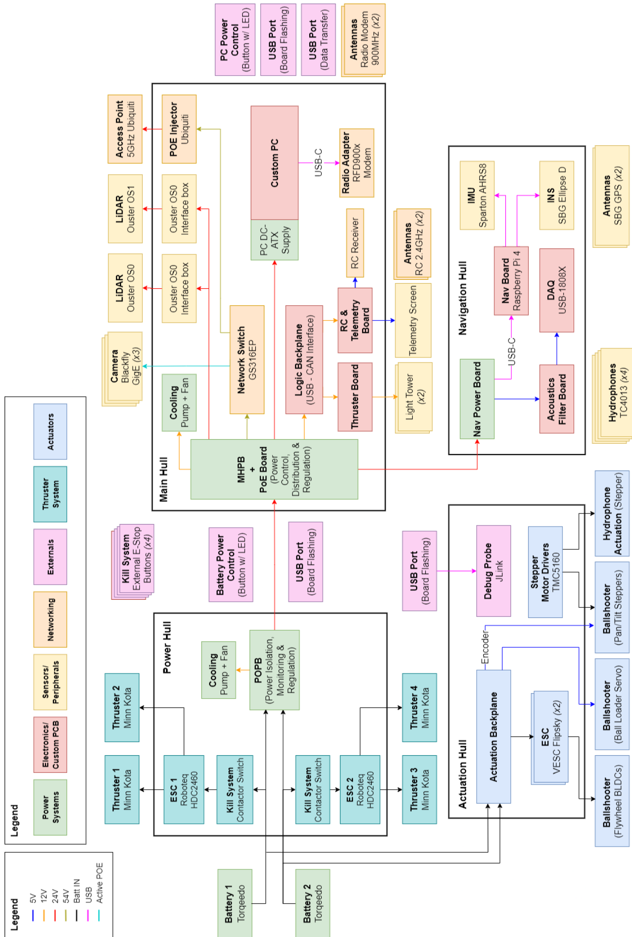
Fig. 26: Electrical power (intra-ASV) architecture.
