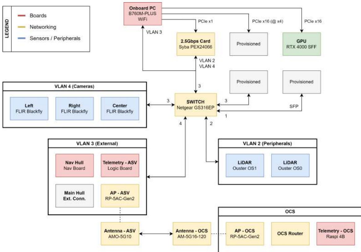
Fig. 24: Intra-ASV network architecture.
