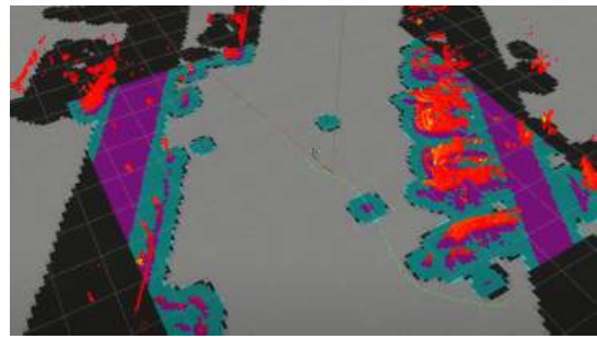
Fig. 10: LiDAR point cloud (red) and local costmap (purple) demonstrates the vehicles mapping and navigation capabilities.
