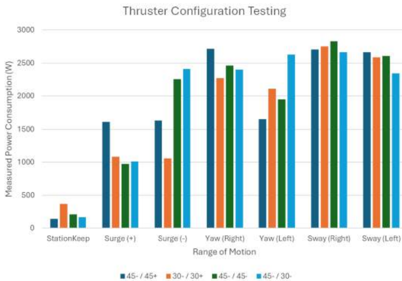
Fig. 22: Comparison of power consumption across thruster configurations.
