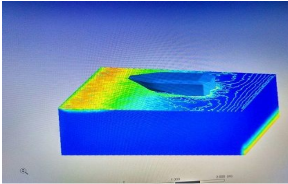
Fig 3 CFD analysis of Poseidon in ANSYS Fluent
