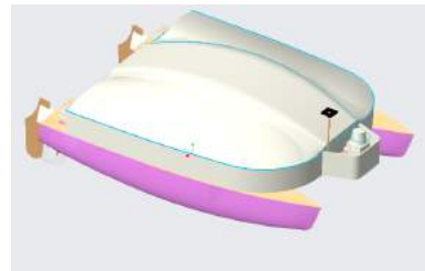
Fig. 9. Electronics Compartment Cover Modeled in PTC Creo
