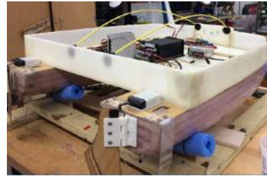
Fig. 8. New Catamaran Center with two pole Framework
