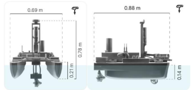
Fig. 2 Nala Theseus Principal Dimension
