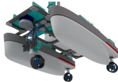
Fig. 3 Propulsion system
