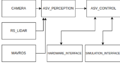
Fig. 6 Nala Theseus Software Architecture
