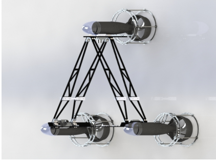
Fig. 9: Surge Mount CAD
