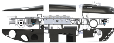
Fig. 14: Surface Exploded View
