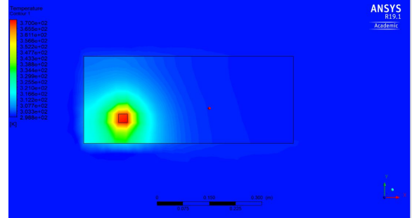
Fig. 7: Temperature Distribution of the Base-plate
