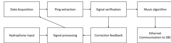
Figure 7: Acoustics flow diagram
