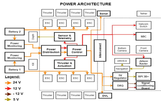
Figure 6: Power architecture block diagram
