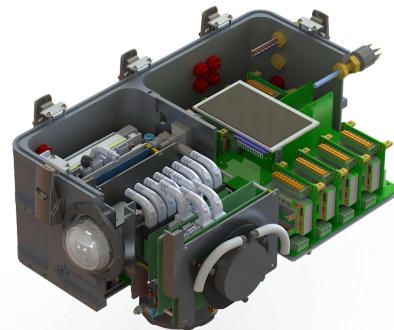
Figure 2: Internal layout of main hull
