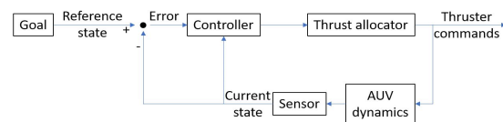
Figure 8: High-level design of AUV controls
