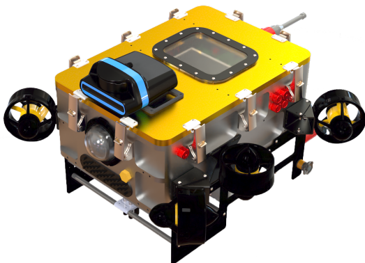
Figure 1: 3D model of BBAUV 4.0
