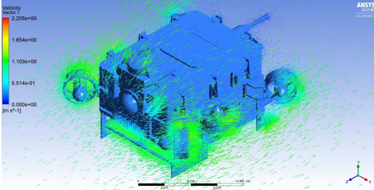
Figure 9: Flow analysis in ANSYS Fluent
