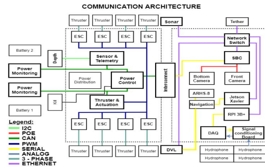
Figure 5: Communication architecture block diagram
