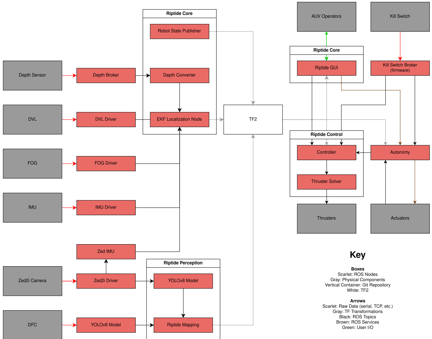
Fig. 28: Riptide Software Architecture Diagram
