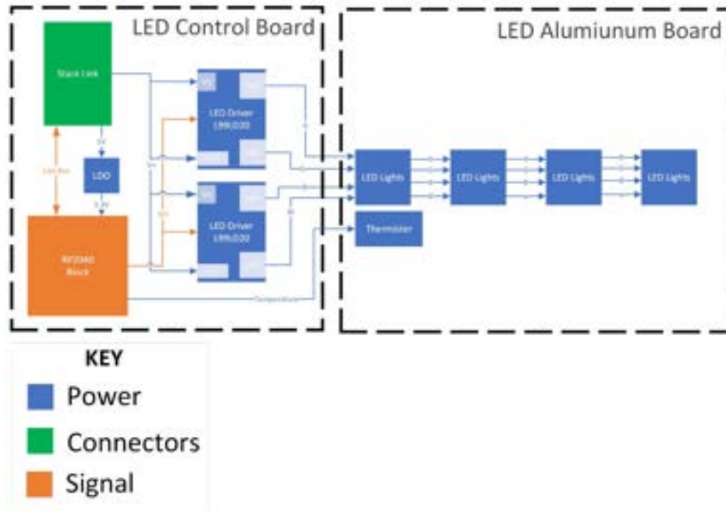
Fig. 26: LED Electrical Block Diagram
