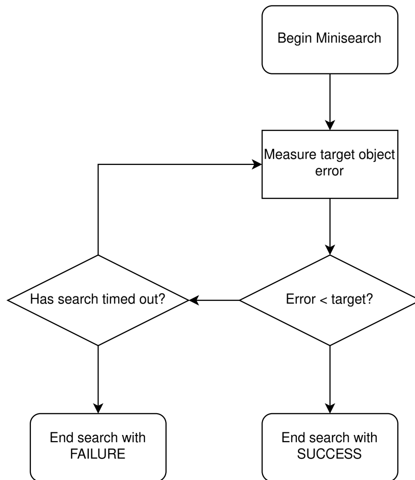
Fig. 16: Autonomy miniature search algorithm flow chart
