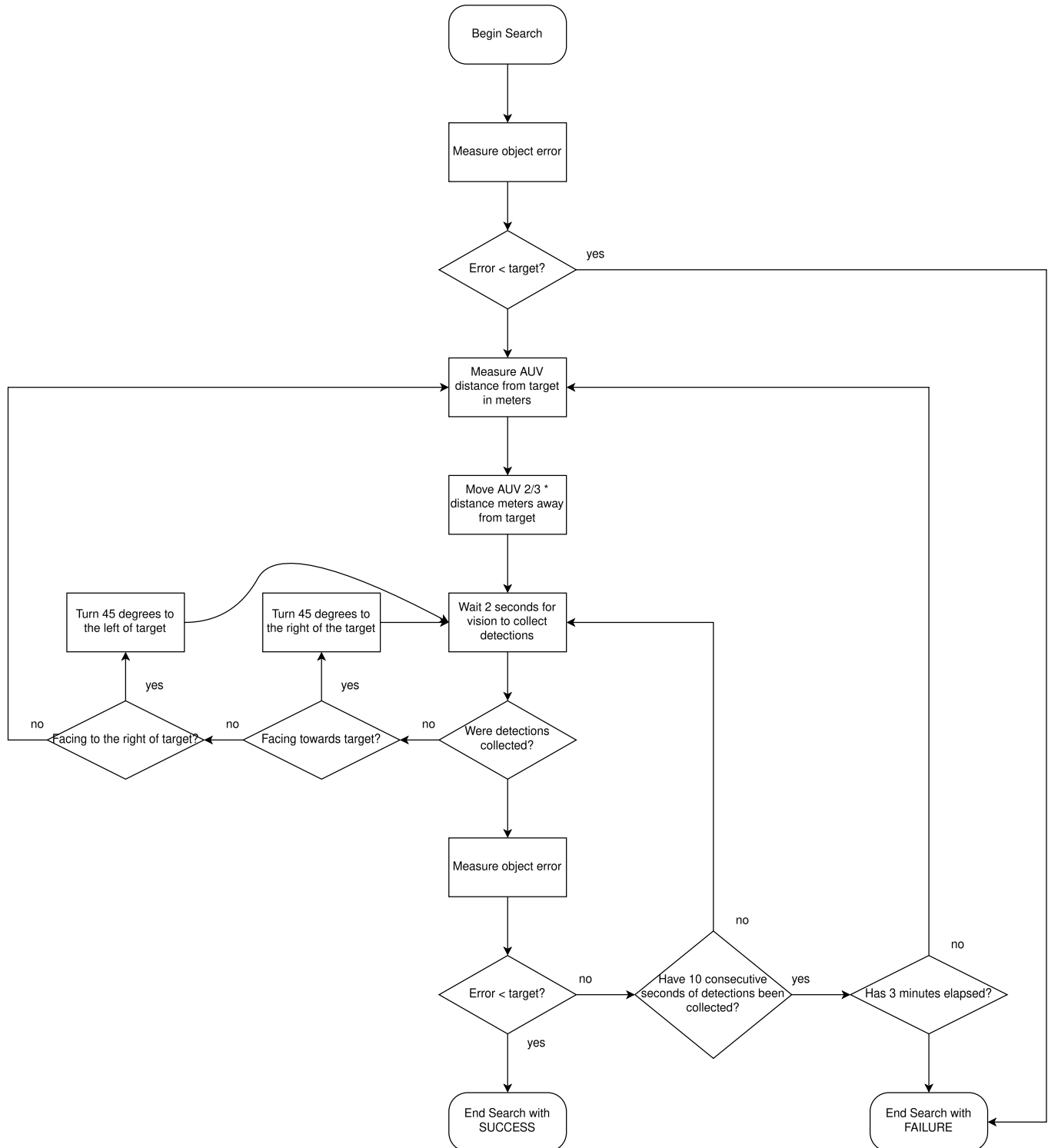
Fig. 14: Autonomy Search algorithm flow chart
