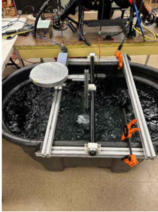
Fig. 8: The apparatus used to characterize the thrusters
