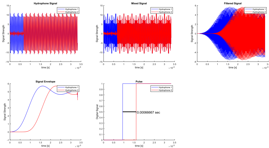
Fig. 19: Acoustics Sample Waveforms
