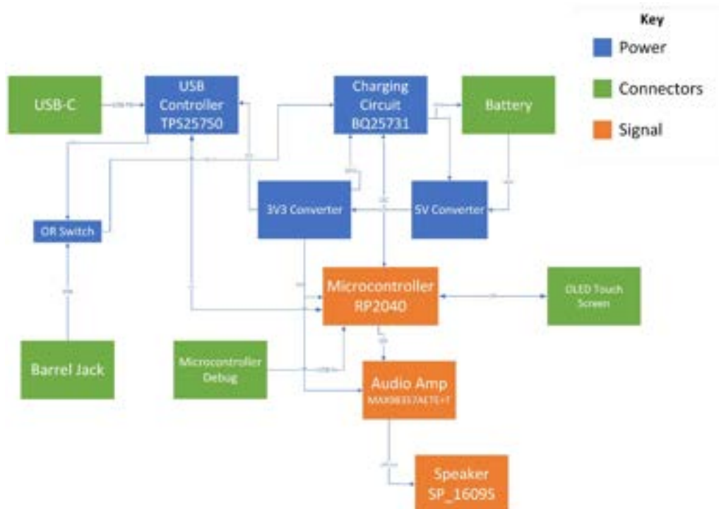
Fig. 27: Smart Battery Charger Electrical Block Diagram
