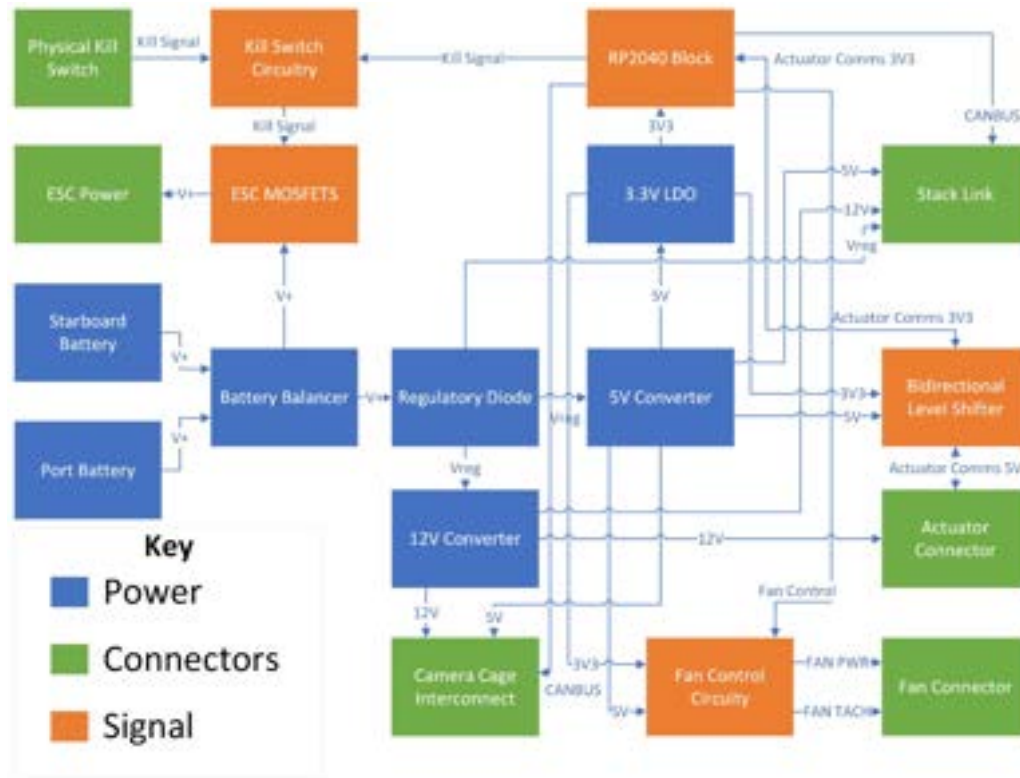
Fig. 24: Poactuator Electrical Block Diagram
