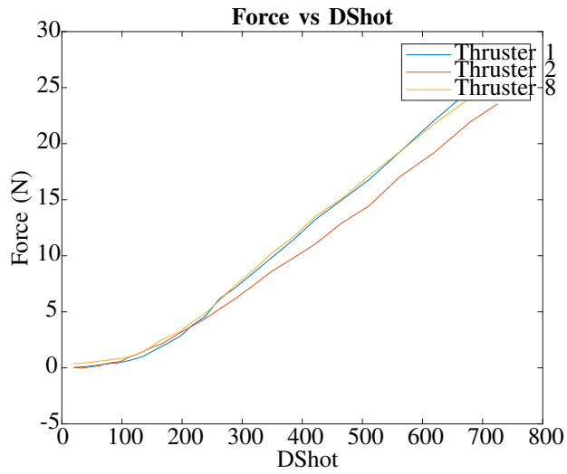
Fig. 9: Force vs Dshot command for three Blue Robotics T200 thrusters.
