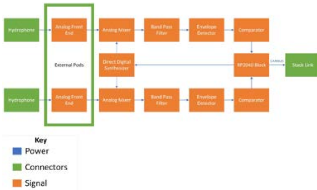
Fig. 25: Acoustics Electrical Block Diagram
