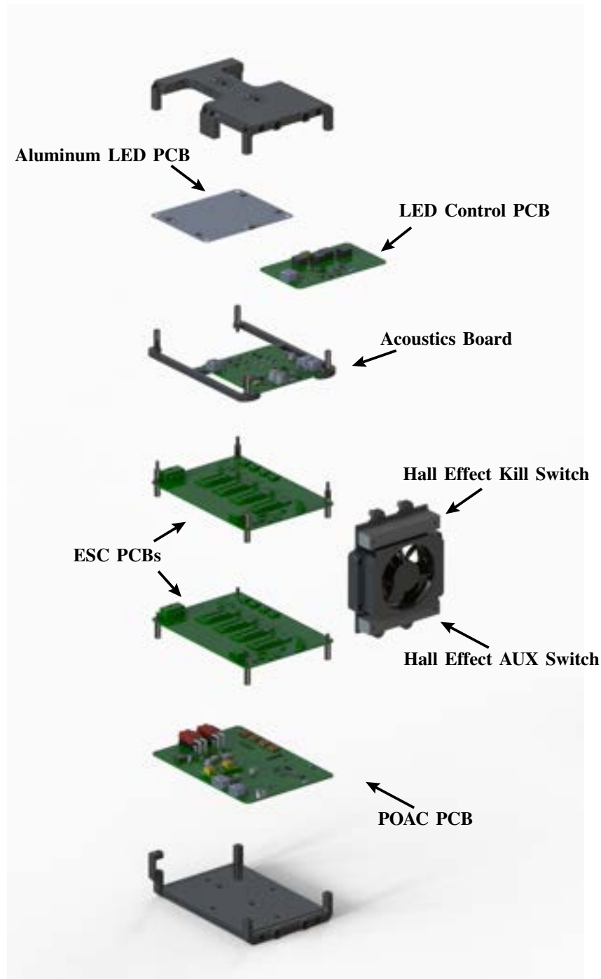
Fig. 17: Board Cage Exploded View
