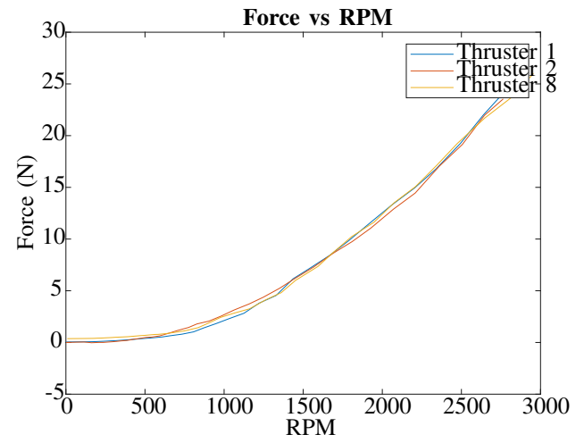
Fig. 10: Force vs RPM for the same Blue Robotics T200 thrusters as in fig. 9
