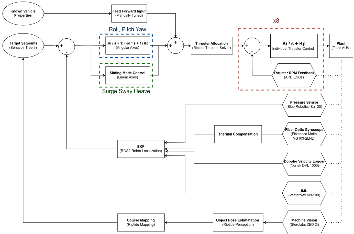
Fig. 30: The positional control feedback diagram
