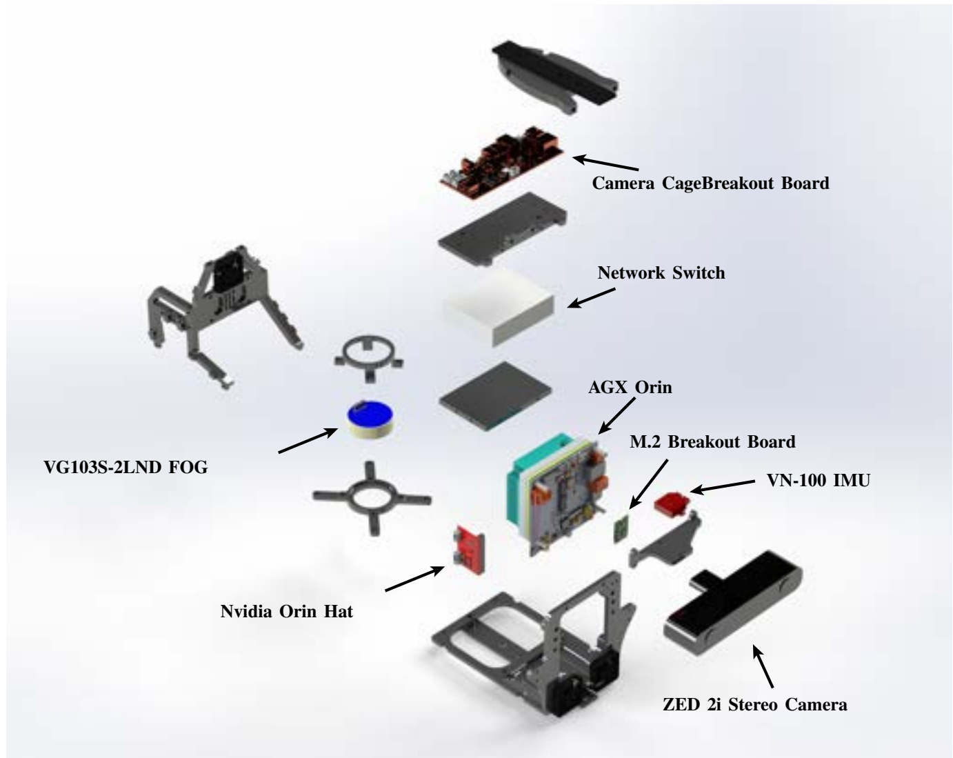
Fig. 18: Camera Cage Exploded View
