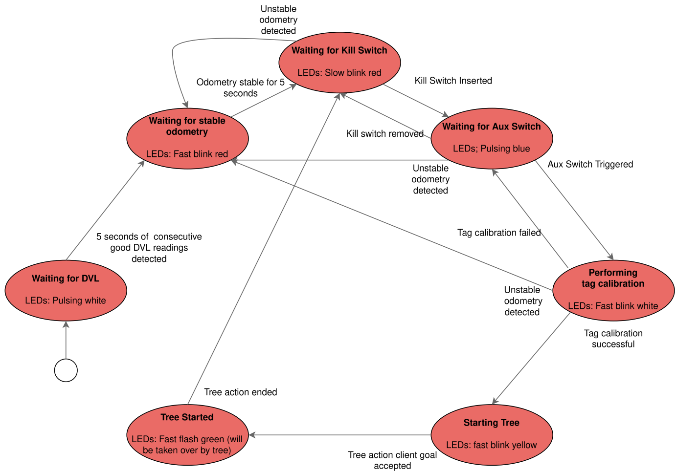
Fig. 29: The state diagram of the AUV headless interface
