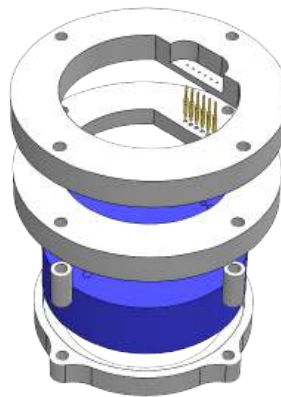
Fig. 18: FOG Mount Exploded Assembly
