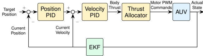
Fig. 12: Control system block diagram.
