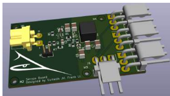
Fig. 28: 3D Render of Actuator Power Distribution Board
