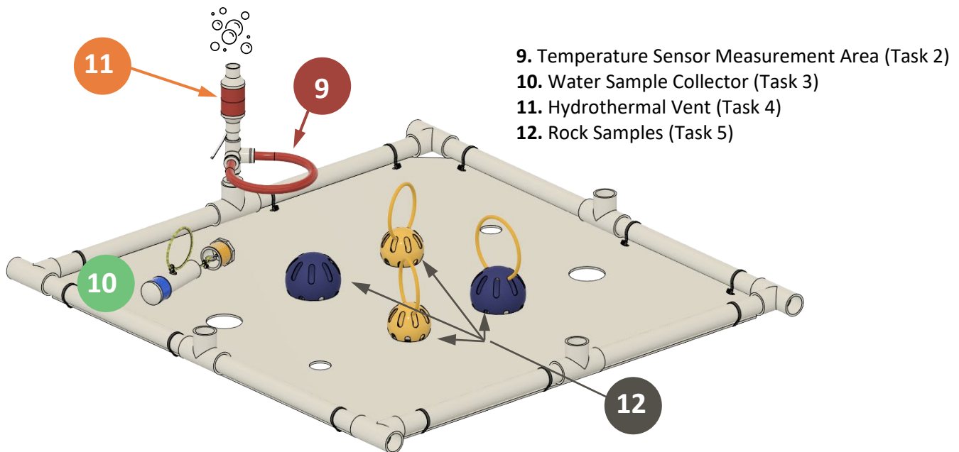
Ocean Bottom Platform with Task Elements
